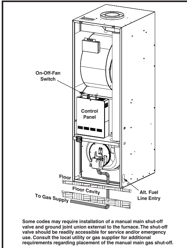
Figure 2. MG1 Gas Furnace Components
