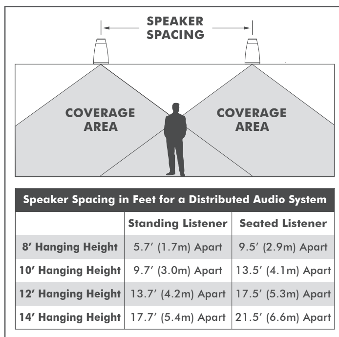
FIGURE 2: SPEAKER SPACING
