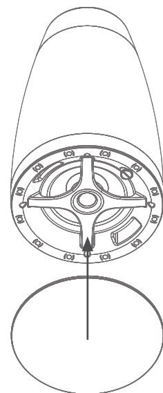
FIGURE 21: GRILLE INSTALLATION
