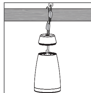
FIGURE 8: SECONDARY SUPPORT
