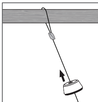
FIGURE 5: THREAD CABLE
