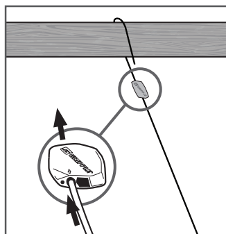
FIGURE 4: THREAD GRIPPLE
