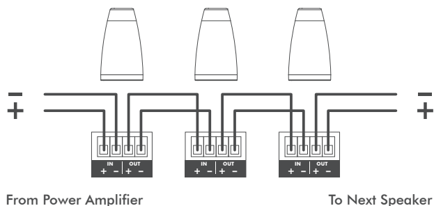
FIGURE 18: LOOP THROUGH CONNECTION
