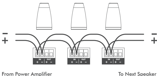
FIGURE 17: PARALLEL CONNECTION
