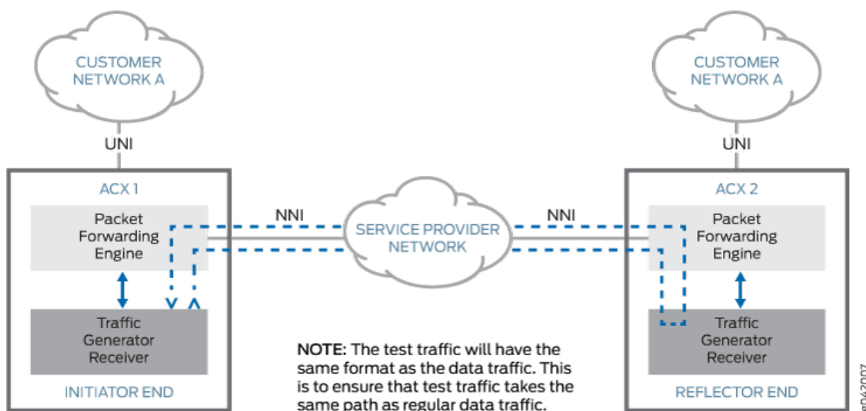
Figure 50: RFC 2544-Based Benchmarking Test Methodology
