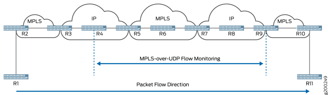
Figure 37: MPLS-over-UDP Over IP-MPLS-IP Network
