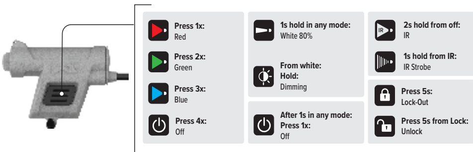
Figure 2 – Switch Operation
