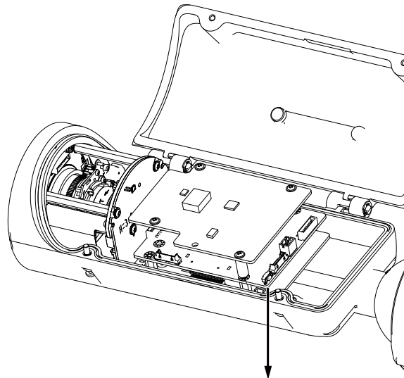
Reset Button
