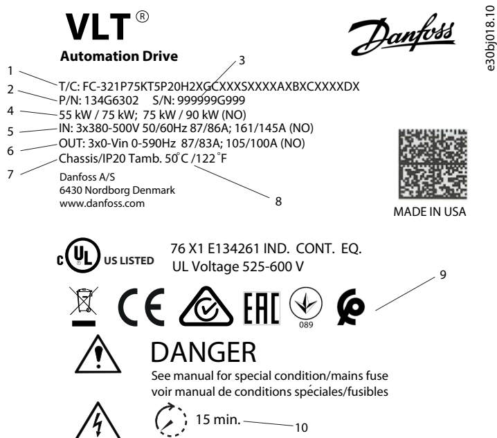
Illustration 1: Nameplate Example
