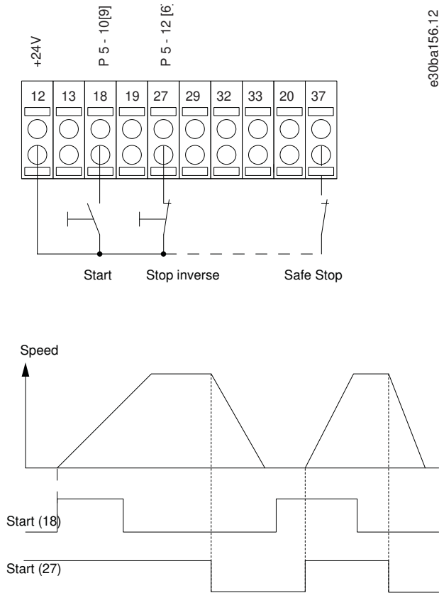
Illustration 7: Pulse Start/Stop
