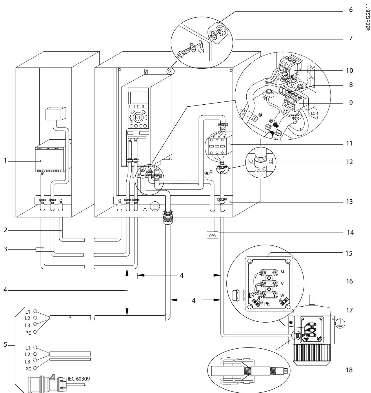
Illustration 4: Example of Proper EMC Installation
