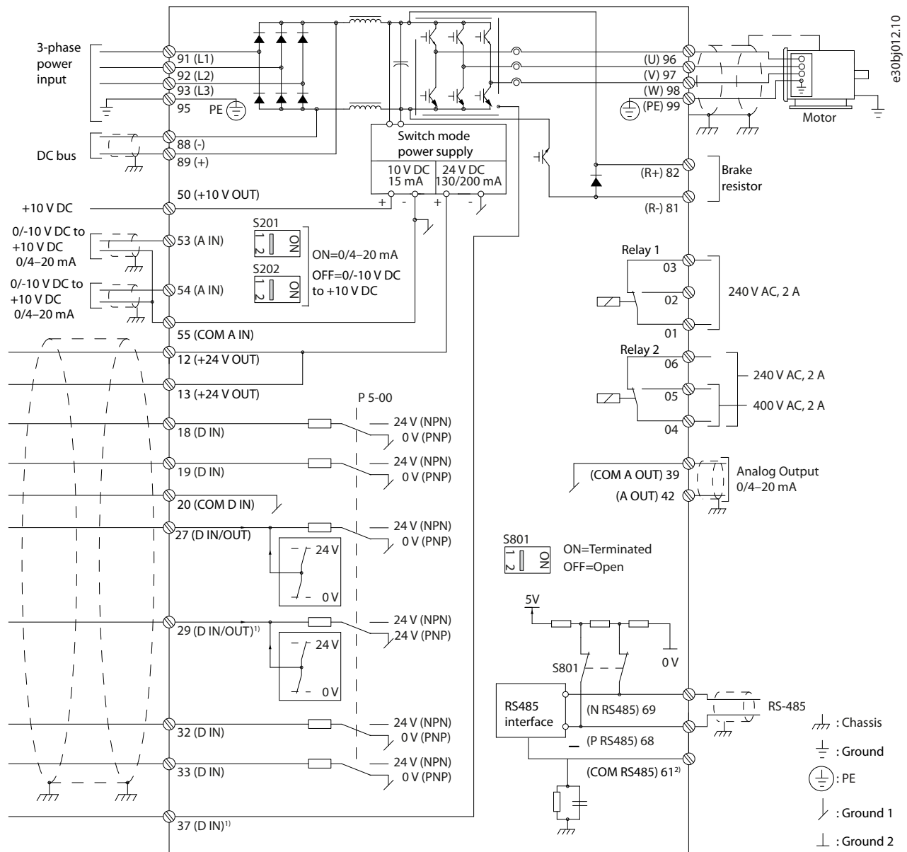
Illustration 5: Wiring Schematic
