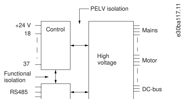
Illustration 12: PELV Isolation
