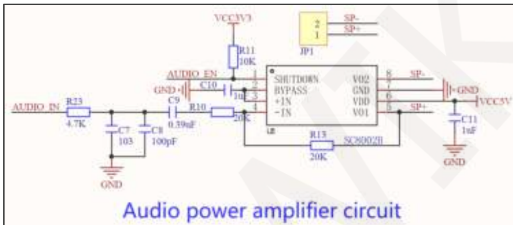
Figure 3.9 Audio power amplifier circuit
