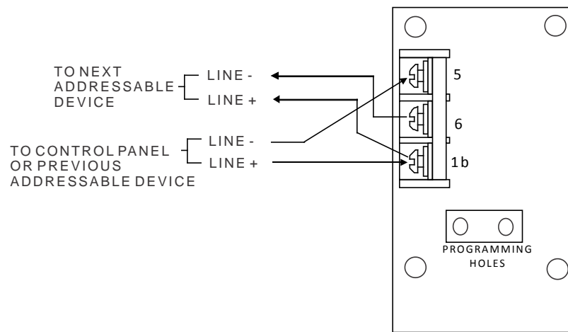
Figure 4 ILED-X isolator mode wiring
