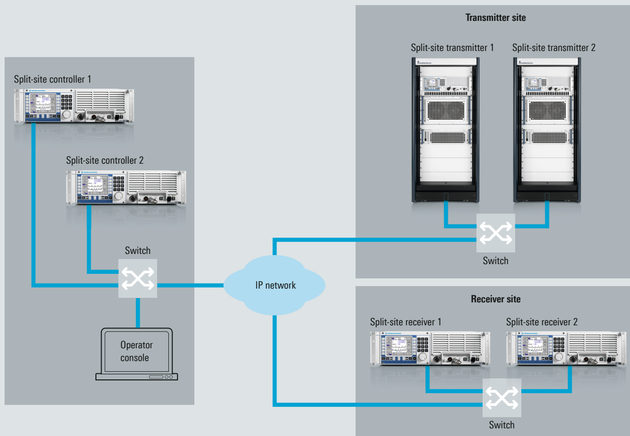
Split-site system with R&S®M3SR Series4100 radios
