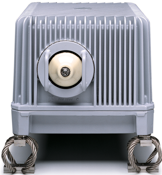
R&S®FK4190M HF antenna tuning unit
