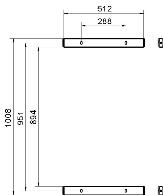
Installation dimensions of fastener strips
