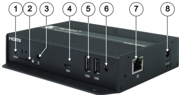
Figure 1: KDS-MP2 Digital Media Player - Front
