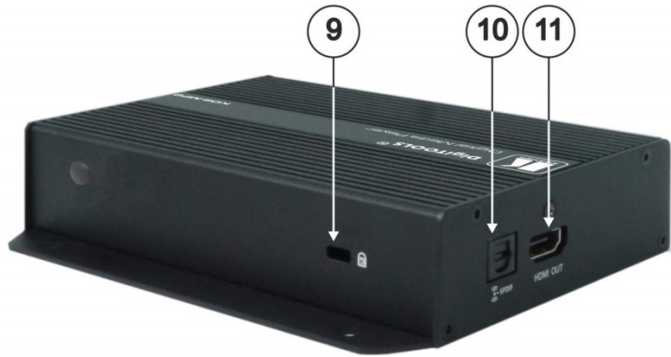
Figure 2: KDS-MP2 Digital Media Player – Rear
