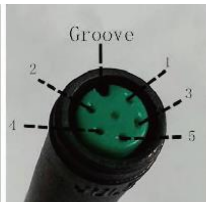
mating connector from controller side
