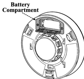
Figure 8: Battery location
