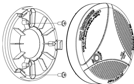
Figure 9: Mounting the bracket
