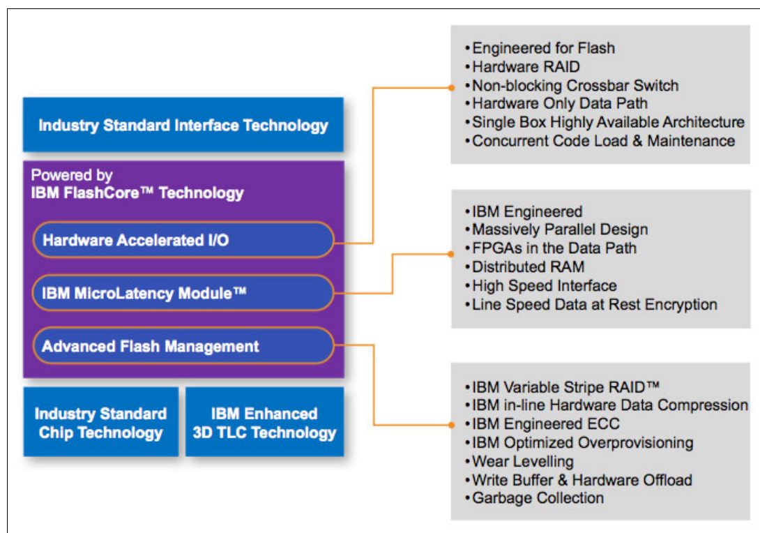
Figure 2 IBM FlashCore Technology
