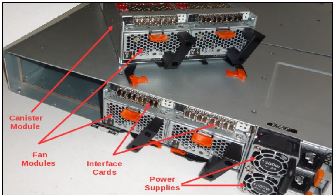
Figure 4 Rear view of IBM FlashSystem 900 Model AE3 with one canister removed
