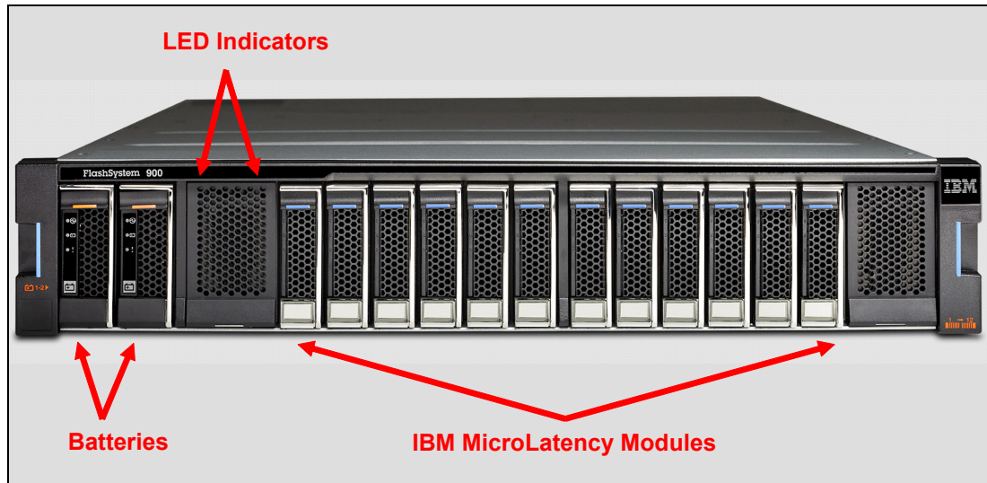
Figure 3 IBM FlashSystem 900 Model AE3 Enclosure Locations
