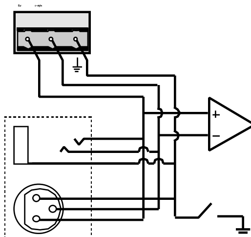
Equivalent Input Schematic - ZR500 Amplifier (Polarity and gain jumpers omitted for clarity.)
