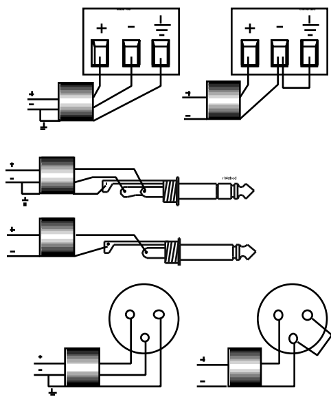
Unbalanced Connections
