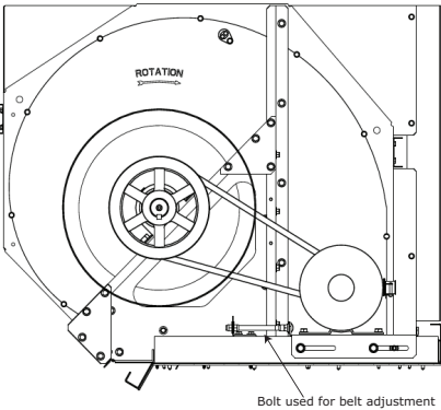
Figure 1. Indoor motor assembly
