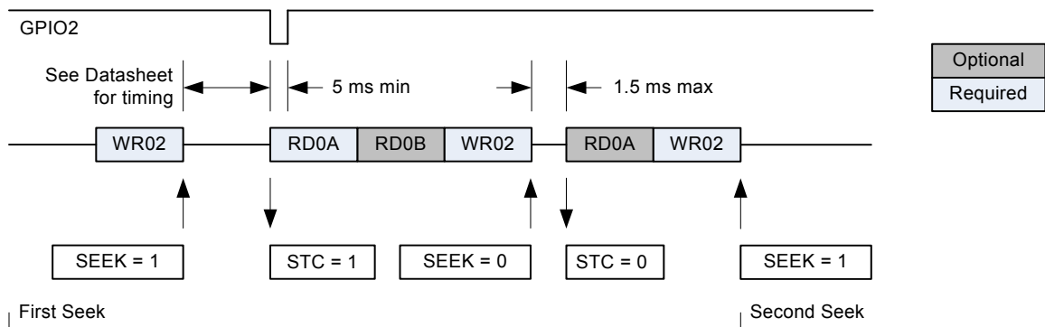
Figure 11. Seek Timing
