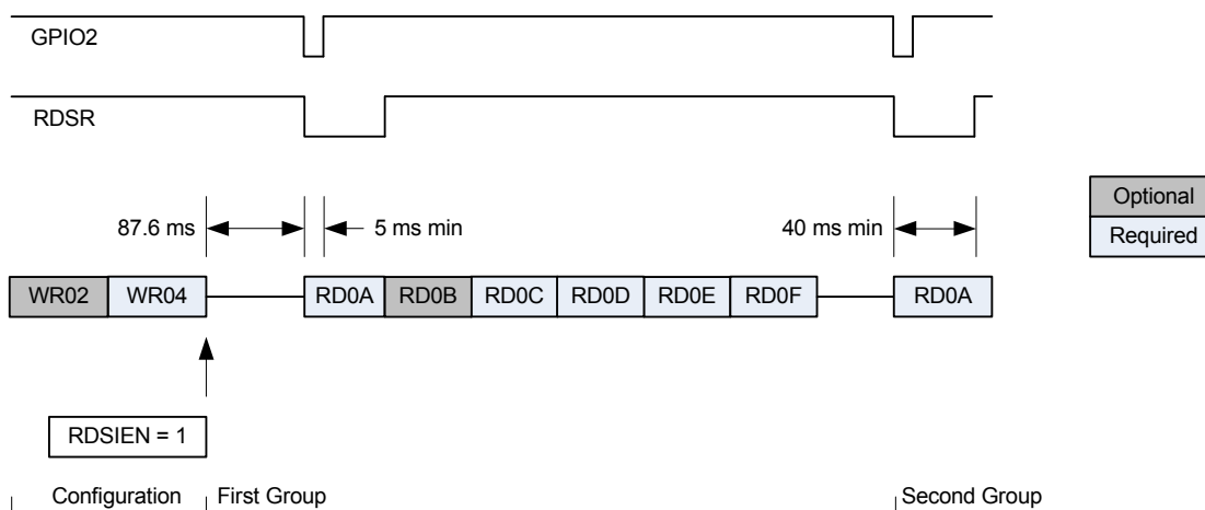
Figure 15. RDS Timing
