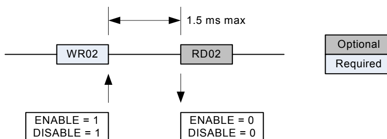
Figure 9. Powerdown Timing
