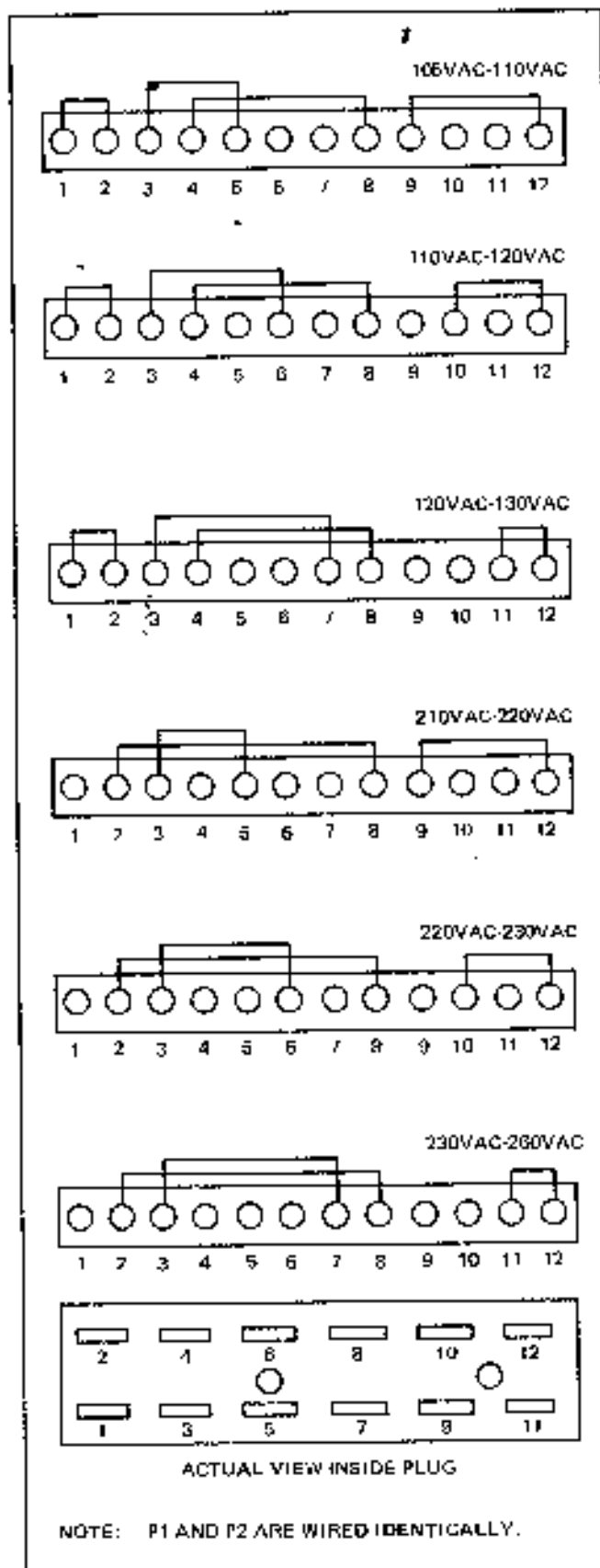
Figure 3.3 Phugs P1 and P2 Installation Location and Wiring Diagram for Various Power Line Voltages
