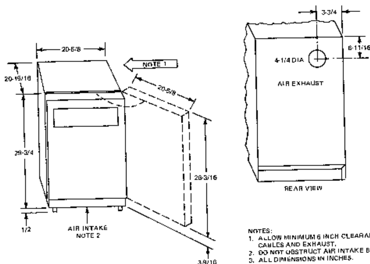
Figure 3.1 RF-103 Outline Dimensions
