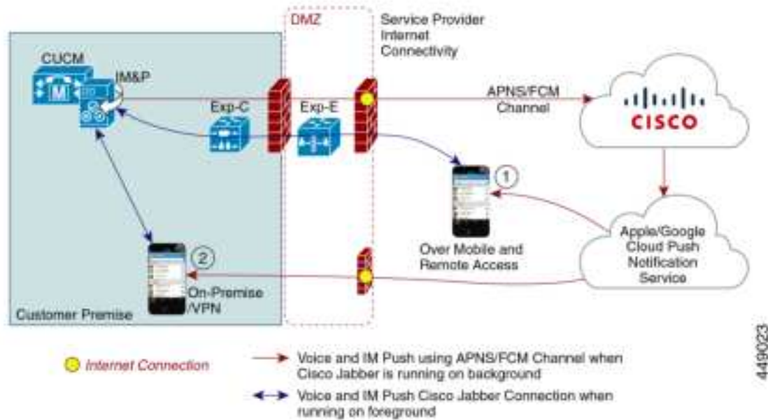
Figure 1: Push Notifications Architecture
