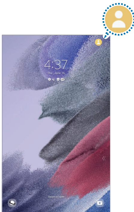
Locked screen
