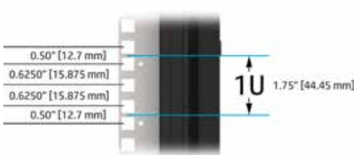
Figure 11. Rack mounting hole positioning in 1U rack space
