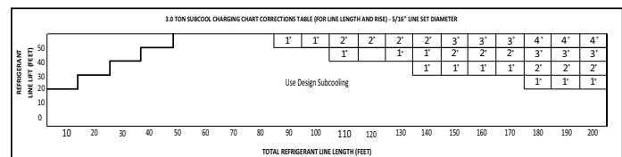
Figure 2. Subcool Charging Corrections – X36 Models
