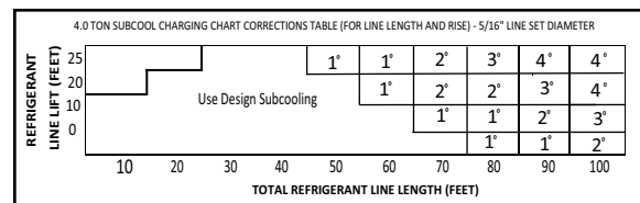
Figure 3. Subcool Charging Corrections – X48 Models
