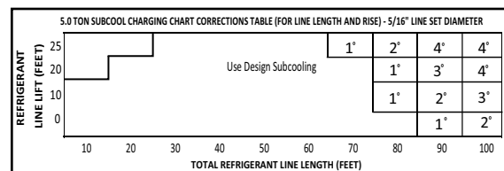
Figure 4. Subcool Charging Corrections – X60 Models (5/16)
