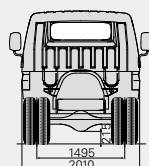
Standard Cab
