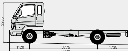
Super Cab Long Wheelbase
