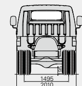
Standard Cab
