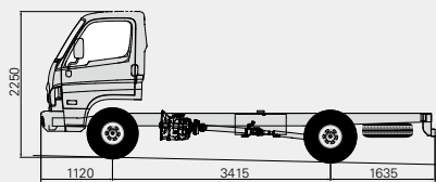
Standard Cab Long Wheelbase
