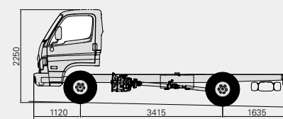
Standard Cab Long Wheelbase (Low)
