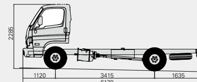
Standard Cab Medium Wheelbase
