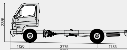
Standard Cab Long Wheelbase
