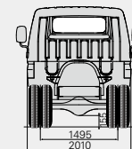
Standard Cab (Low)
