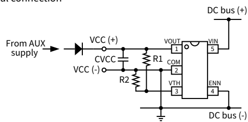
Typical connection
