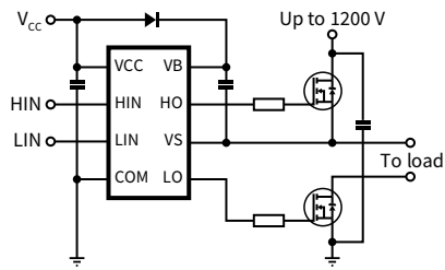
Typical connection
