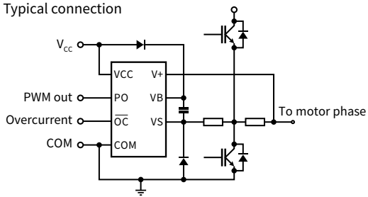
Typical connection
