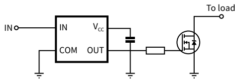
Typical connection
