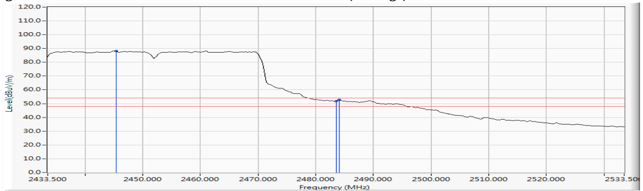
Figure Channel 09:
