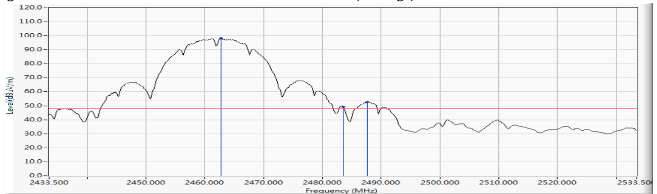
Figure Channel 11:
