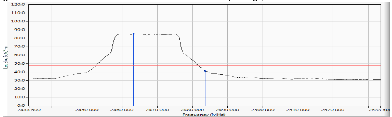
Figure Channel 12:
