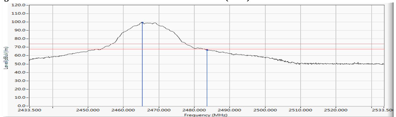
Figure Channel 12:
