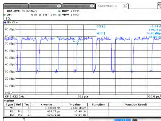
802.11n-40:
