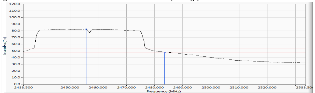
Figure Channel 10:
