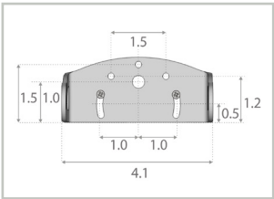
Bracket dimensions
