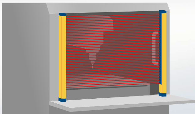
Fig. 4 Safeguarding hazardous points with a safety light curtain
