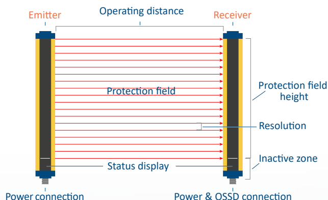
Fig. 3: Safety light curtain - structure & selection criteria
