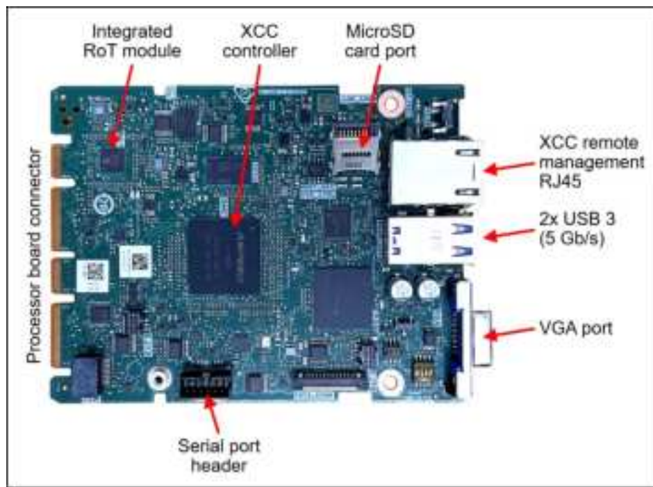
Figure 20. System I/O Board
