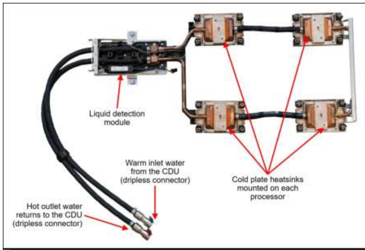
Figure 9. Lenovo Processor Neptune Core Module
