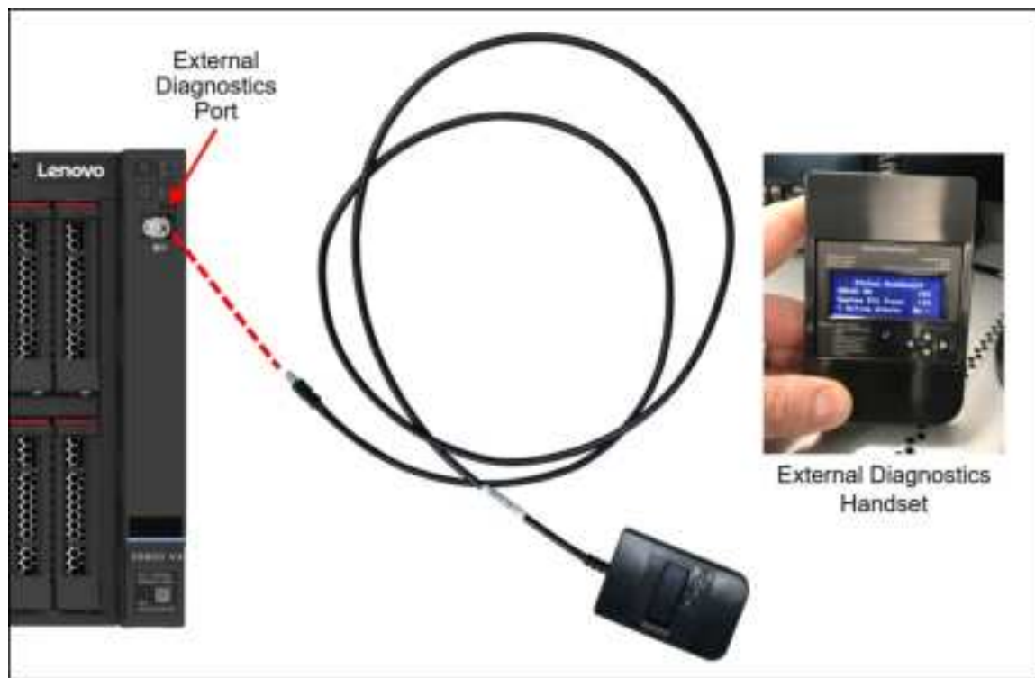
Figure 22. External Diagnostics Handset
