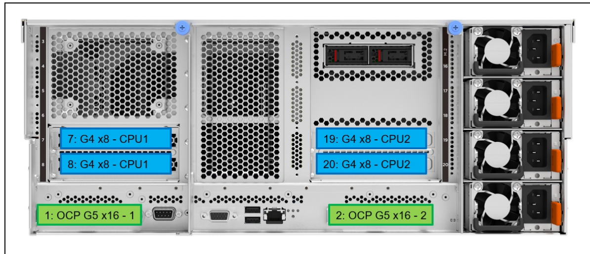
Figure 17. Slot configuration with 4x Gen4 slots
