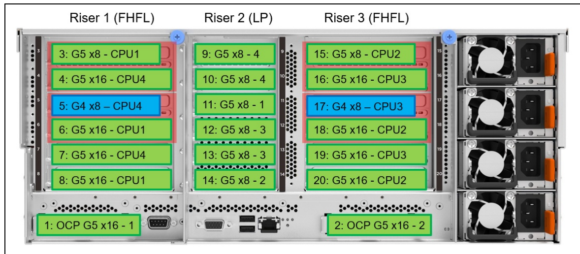
Figure 16. Slot configuration with 16x Gen5 slots + 2x Gen4 slots
