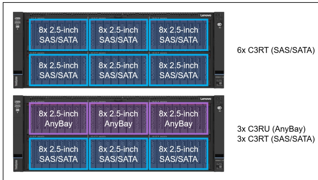
Figure 10. SR860 V4 drive bays - 2.5-inch drive bays
