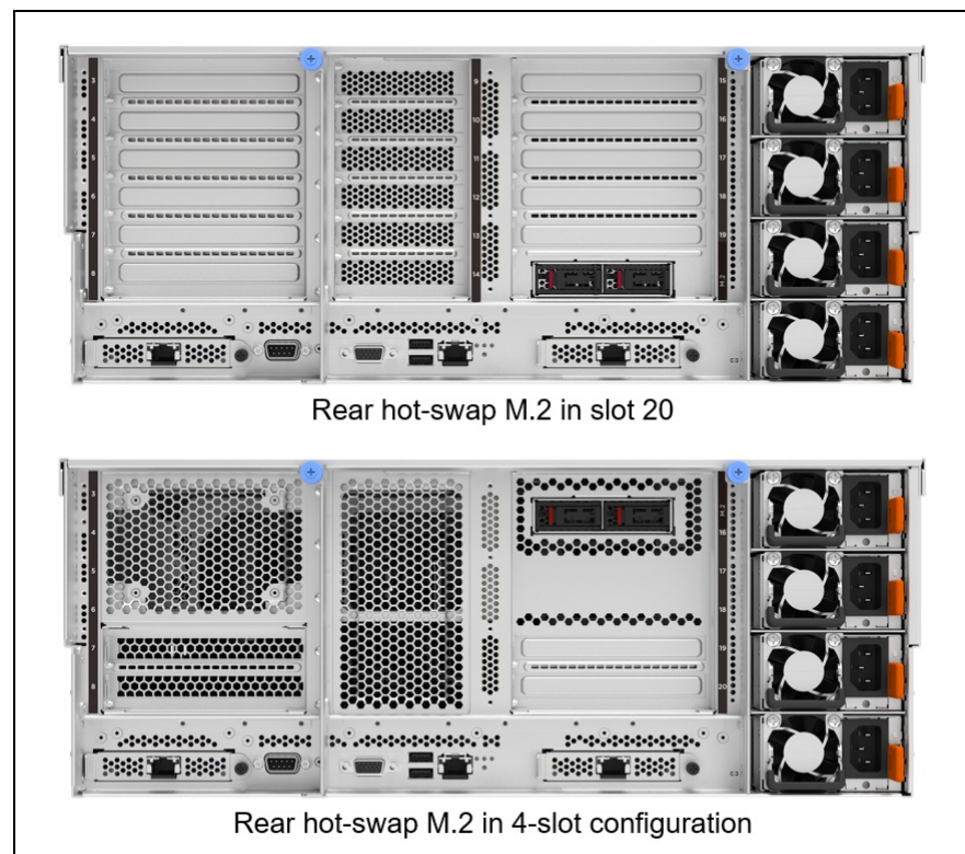
Figure 12. Hot-swap M.2 drive bays
