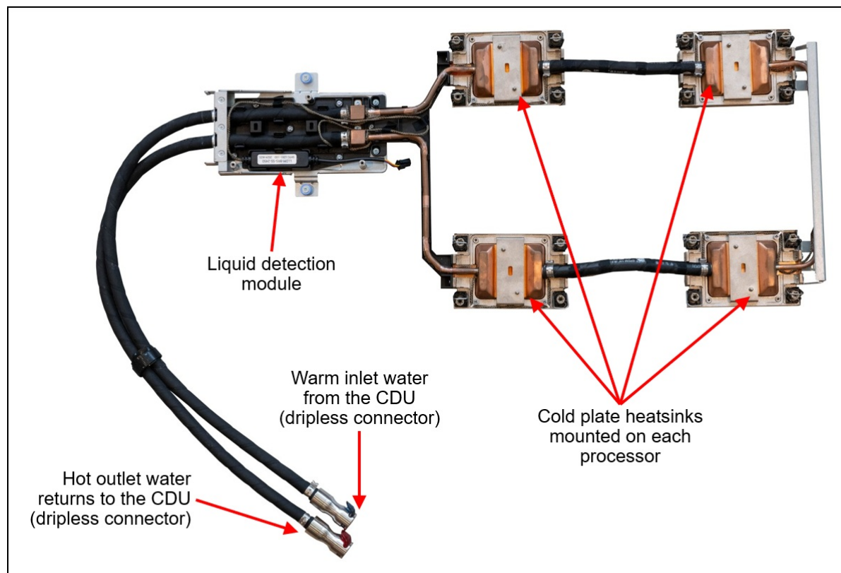
Figure 9. Lenovo Processor Neptune Core Module
