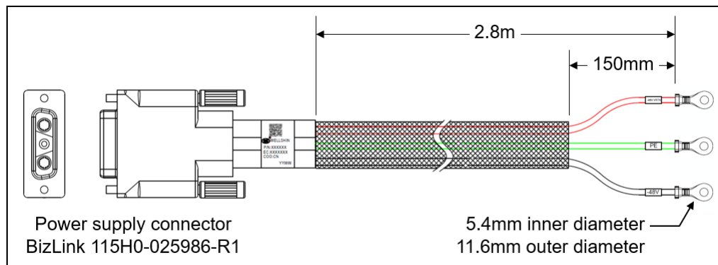
Figure 18. -48V DC power cord
