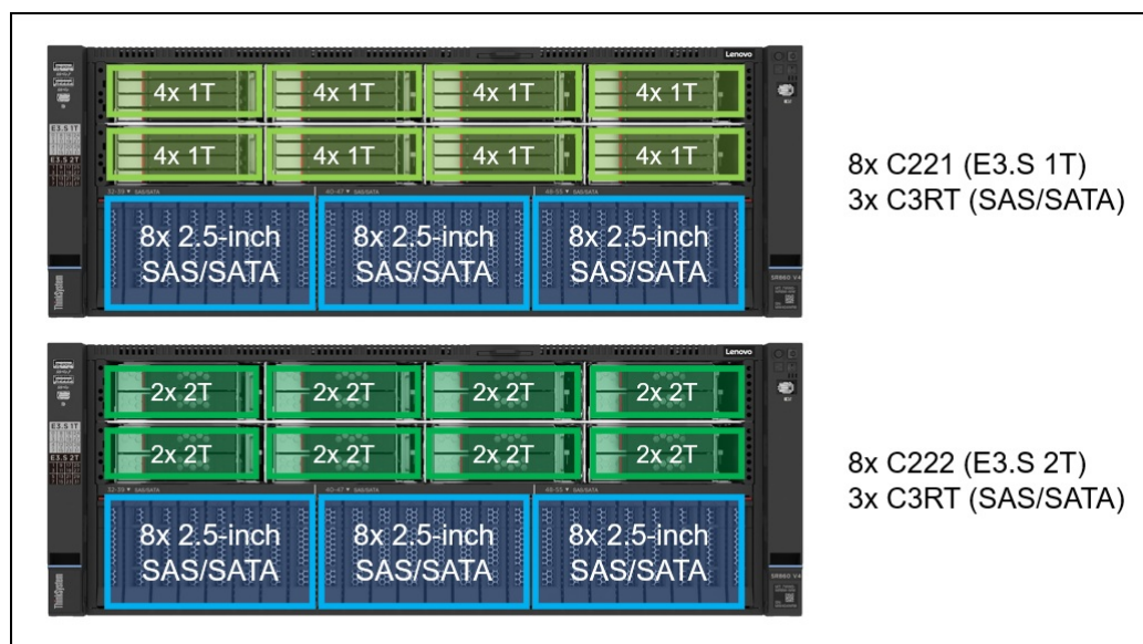
Figure 11. SR860 V4 drive bays - E3.S + 2.5-inch drive bays
