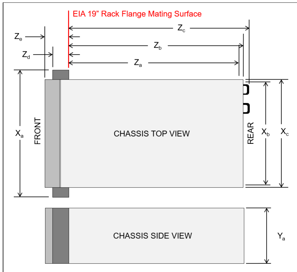
Figure 24. Server dimensions
