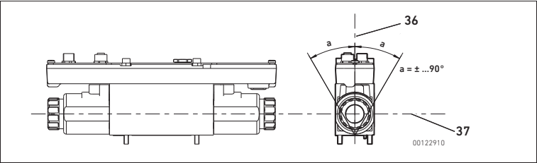
Fig. 3: Mounting orientation
