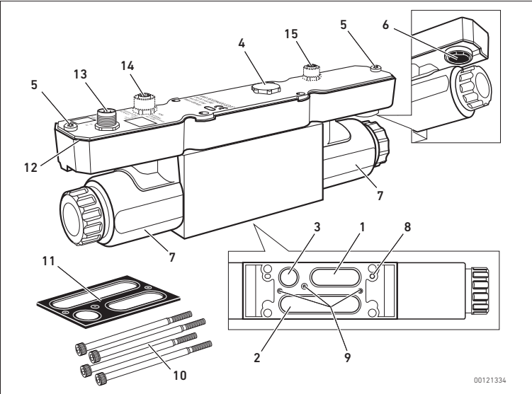
fig 1: Tryckregulator ED07
