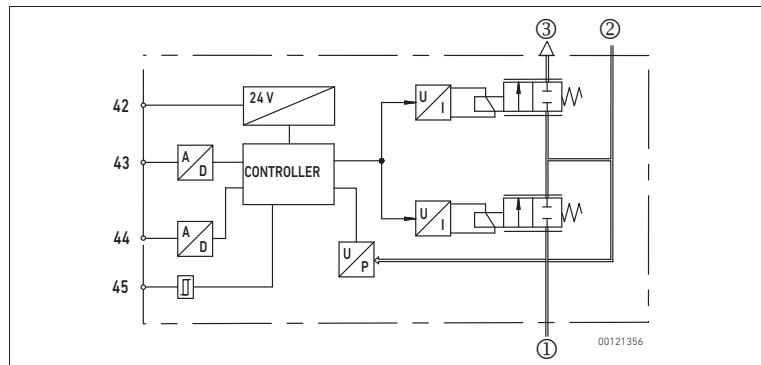
① Inlet connection for supply pressure 42 Supply voltage ② Outlet connection 43 Nominal input value ③ Ventilation 44 Actual output value 45 Switch output
