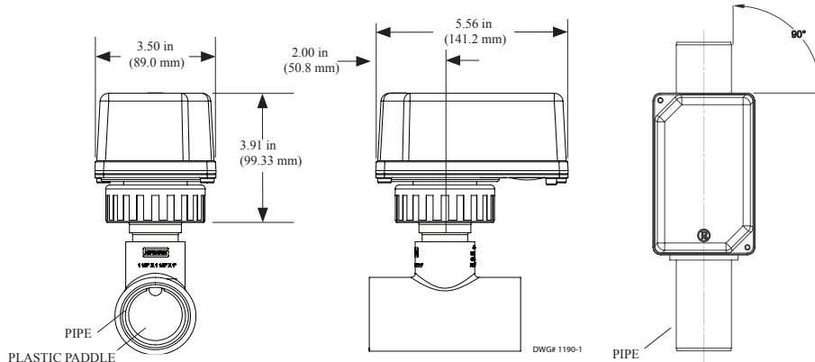
Fig. 7 Mounting Dimensions-Orientation
