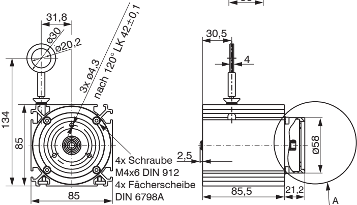
Dimensional drawing wireSENSOR WDS-2500-P85-M, dimensions in mm (inches, rounded off)
