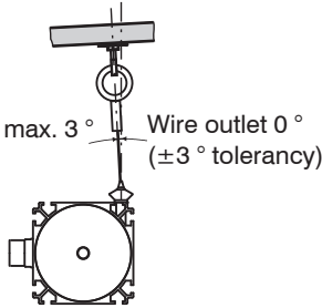
Attachment and maximum diagonal pull of the measuring wire
