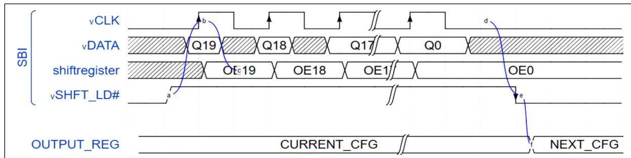
FIGURE 3-14: Side-Band Interface Functional Timing.
