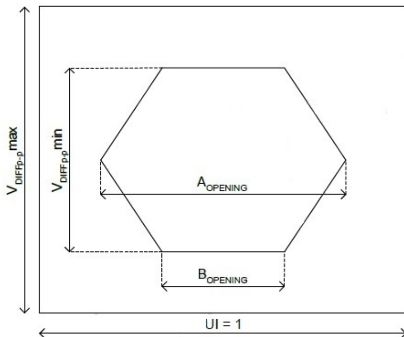
Figure 40. TX and RX eye diagram template
