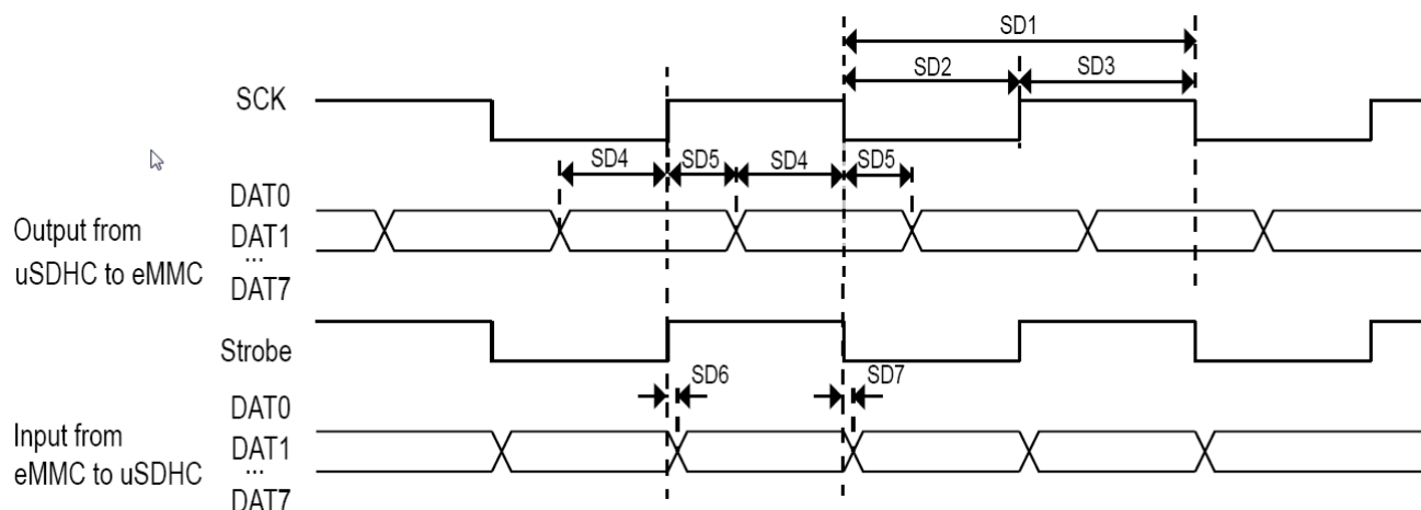
Figure 32. HS400 timing
