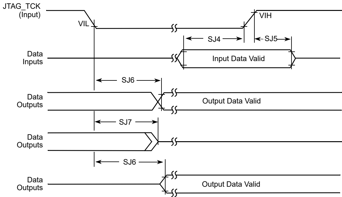
Figure 50. Boundary system (JTAG) timing diagram
