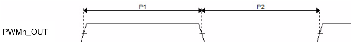
Figure 42. PWM Timing
