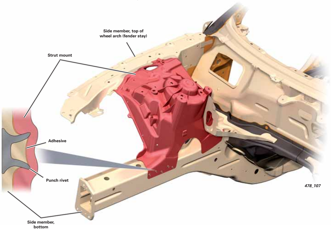
Structural integration of front end and strut mount
