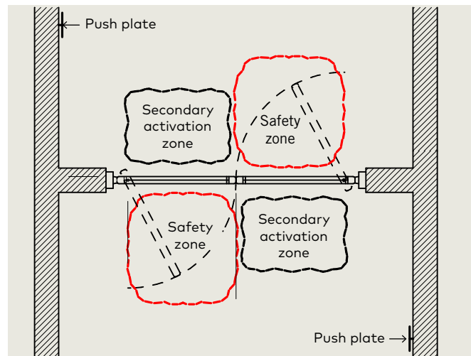
Fig. 5.1.5 Door mounted safety sensors
