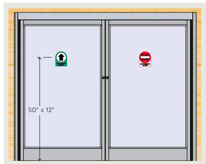
Fig. 7.7.6 LH double egress, exterior side Approach side Swing side
