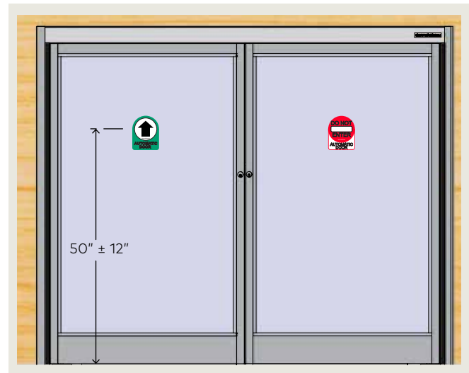
Fig. 7.7.5 LH double egress, interior side Approach side Swing side
