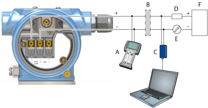
Figure 3-2: 4-20 mA/HART® Communication
