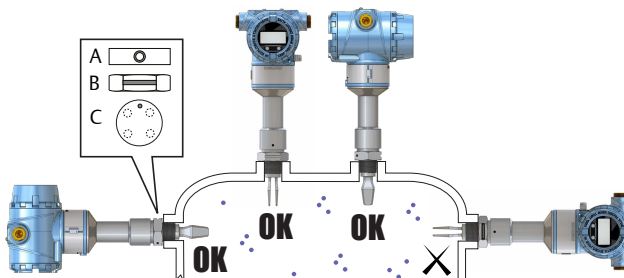
Figure 2-2: Correct Fork Alignment for Vessel (Tank) Installation
