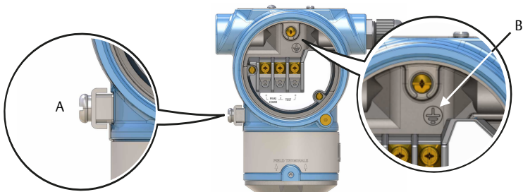
Figure 3-4: Ground Screws
