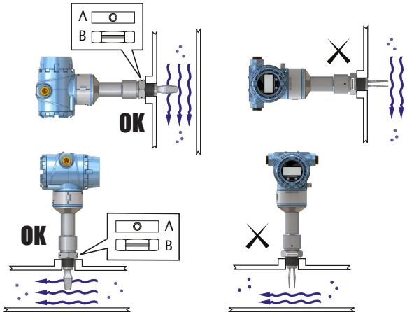
Figure 2-1: Correct Fork Alignment for Pipe Installation
