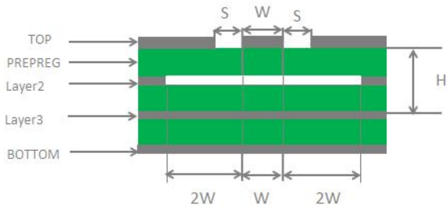
Figure 22: Coplanar Waveguide Design on a 4-layer PCB (Layer 3 as Reference Ground)
