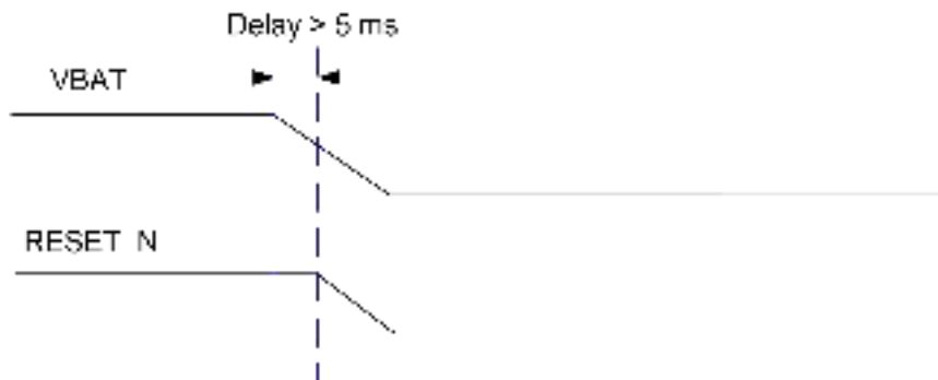
Figure 7: Power-down Timing
