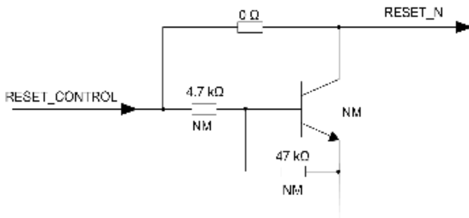
Figure 8: Reference Circuit of RESET_N by Using Driving Circuit
