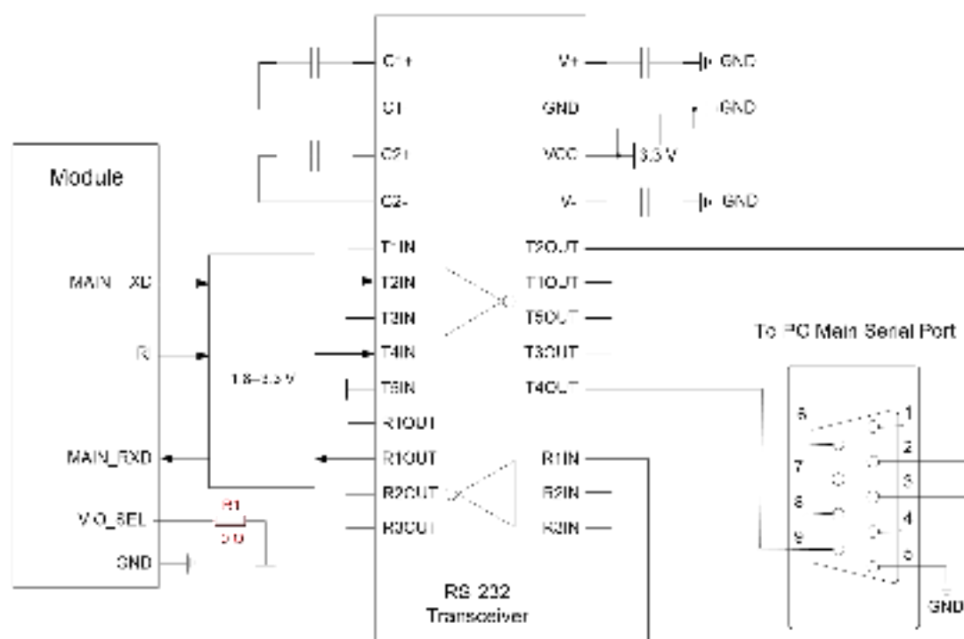
Figure 14: Sketch Map for RS-232 Interface Match
