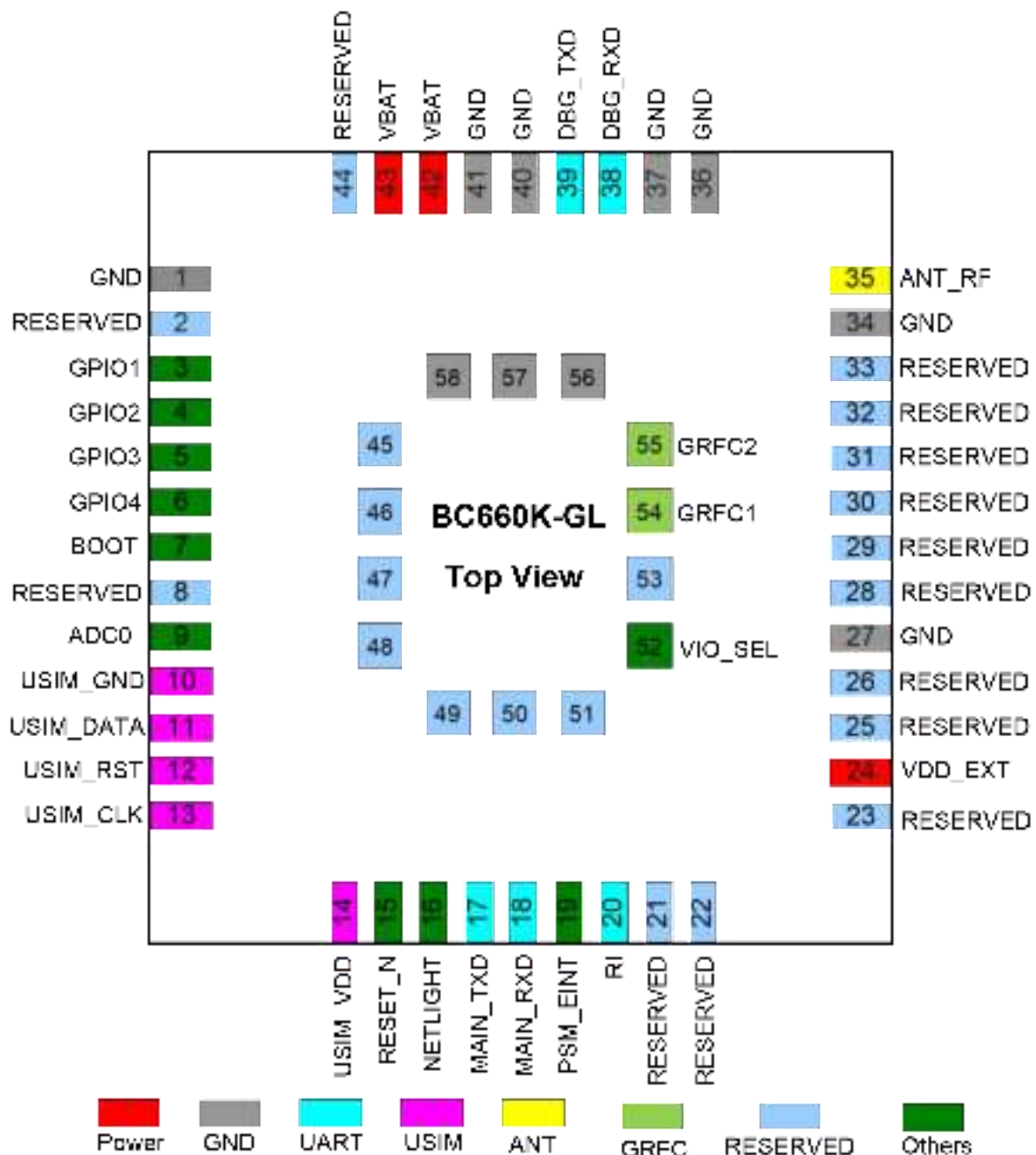
Figure 2: Pin Assignment
