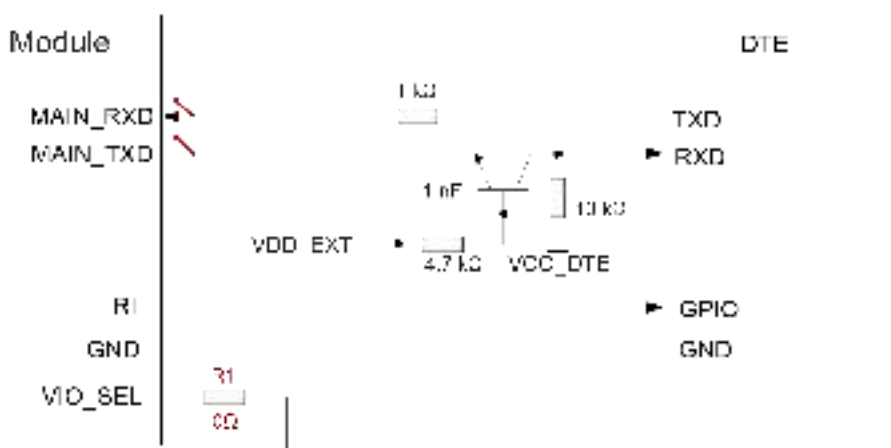
Figure 15: Reference Circuit with Transistor Circuit
