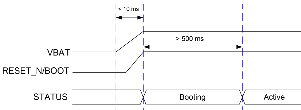
Figure 6: Power-up Timing
