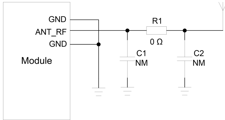
Figure 19: Reference Design of NB-IoT Antenna Interface
