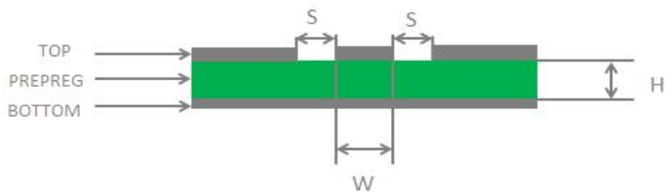
Figure 21: Coplanar Waveguide Design on a 2-layer PCB
