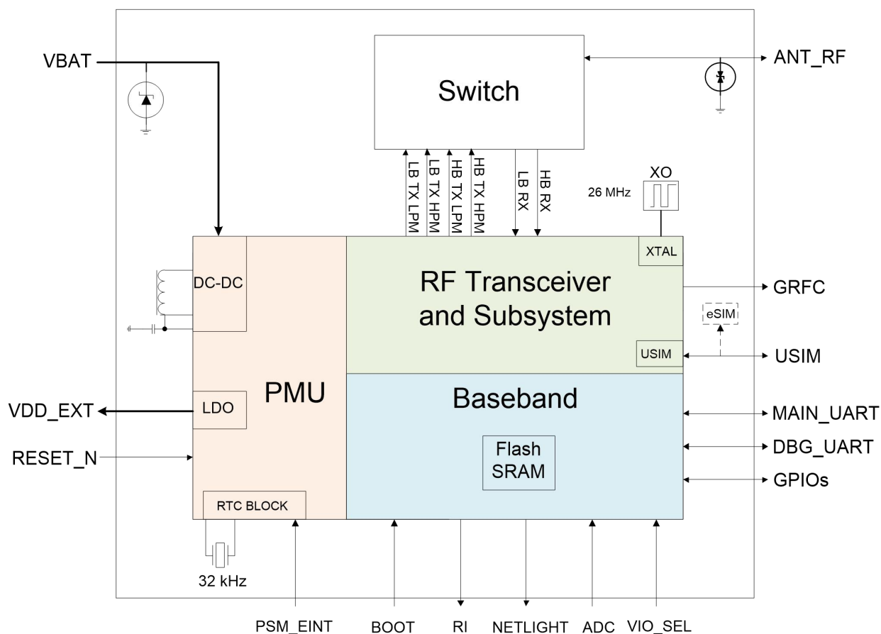
Figure 1: Functional Diagram
