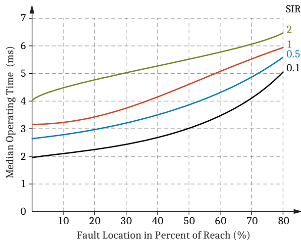
Figure 4 TD21 Element Median Operating Time for Varying Fault Location and Different Source-to-Line Impedance Ratios
