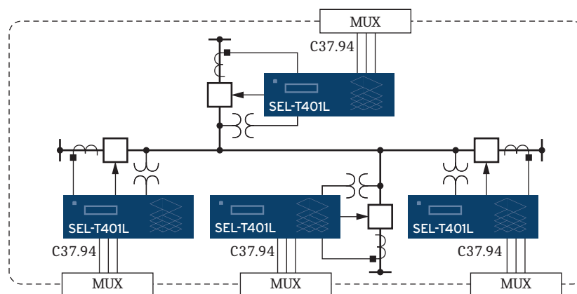
Figure 42 Four-Terminal Line With an IEEE C37.94-Encoded Protection Channel
