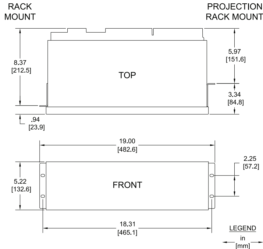
Figure 50 SEL-T401L Rack-Mount Chassis Dimensions
