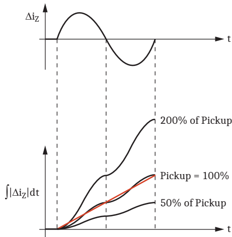
Figure 12 The Incremental Overcurrent Element Principle of Operation
