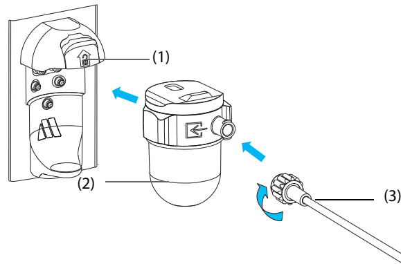
(1) Watertrap receptacle
