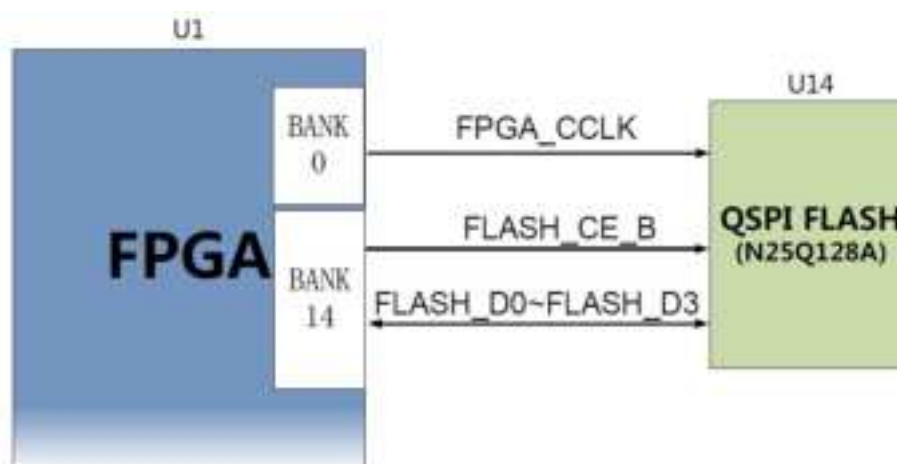
Figure 2.4-1: QSPI Flash Schematic
