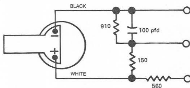
FIGURE 3 — Test Circuit
