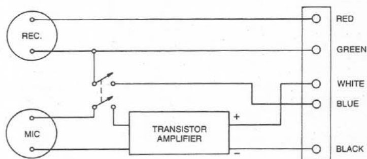
FIGURE 2B — Schematic
