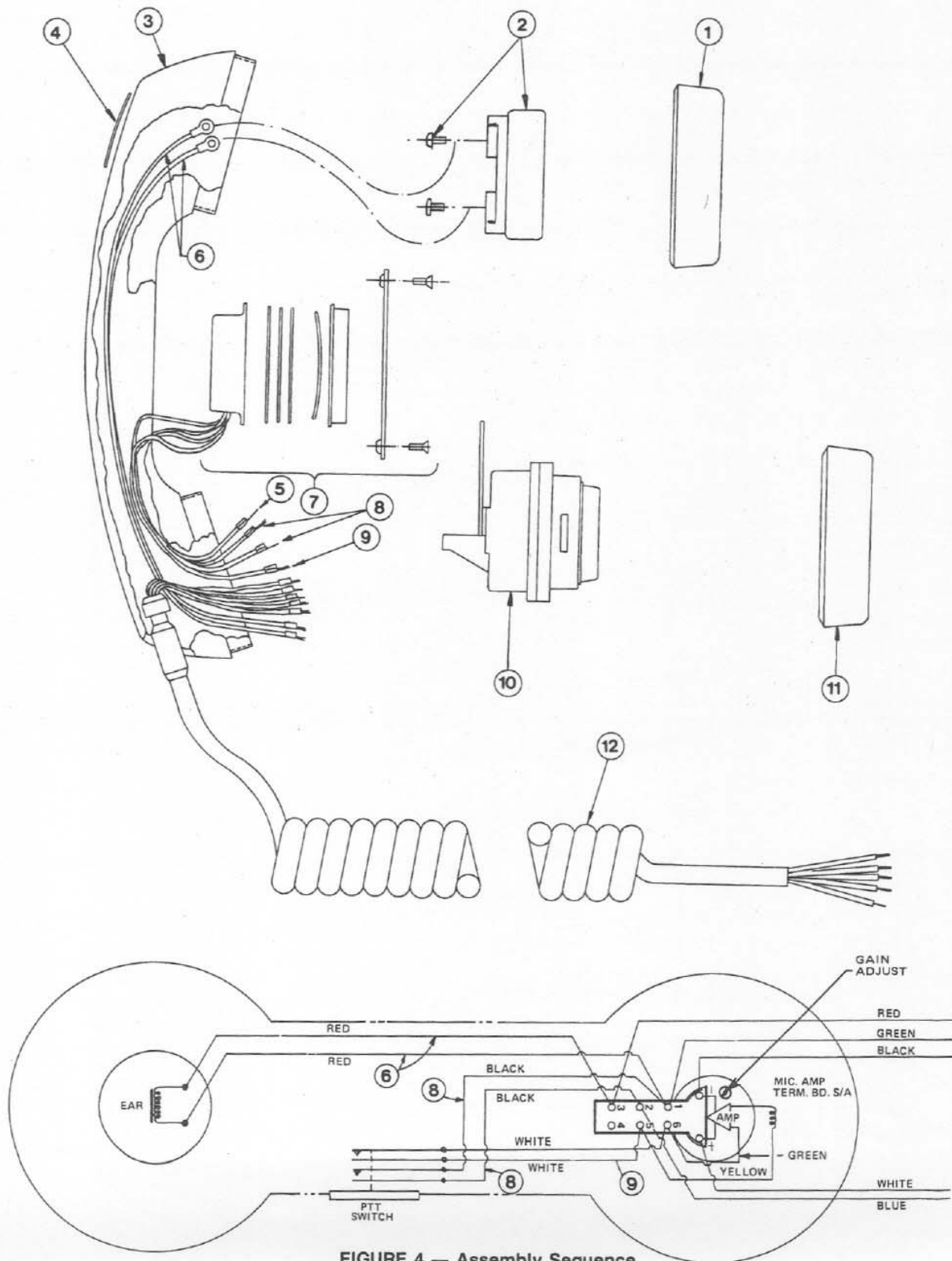
FIGURE 4 — Assembly Sequence
