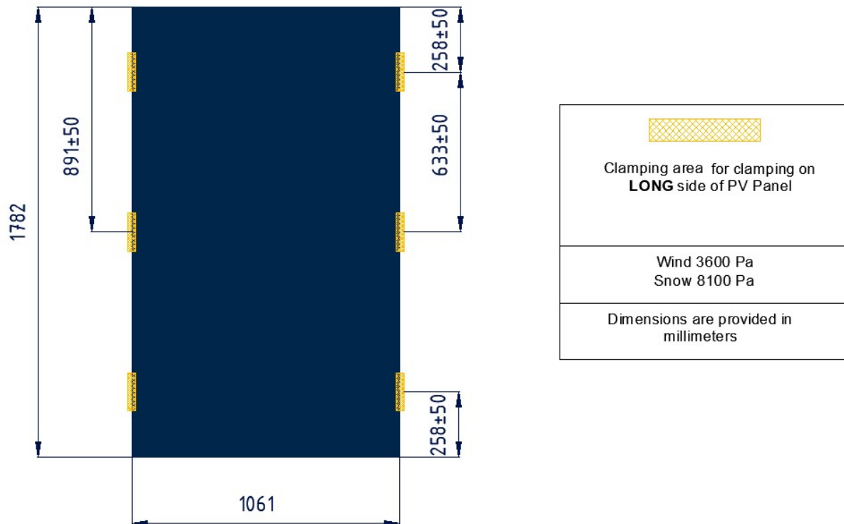
Figure 9. BLACKSTAR B.60(40) mounting with six fixing points on module's long sides
