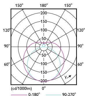
Light Distribution Diagram - 24T5HO/COR/46-835/IF33/G/DIM 25/1
