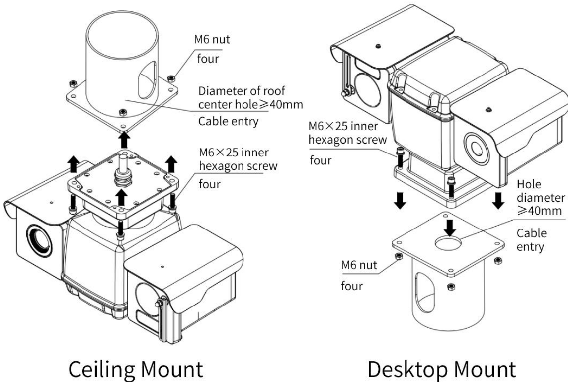
Figure 2.2 Installation Illustrations
