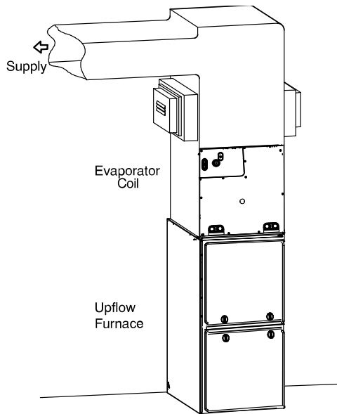
Fig. 16 – Humidifier Application
