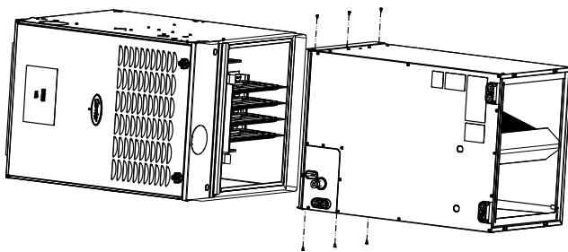
Fig. 10 – Horizontal Right Installation
