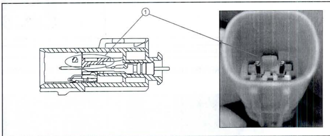
Figure 53. Fully Locked Position (after Wire Installed)
