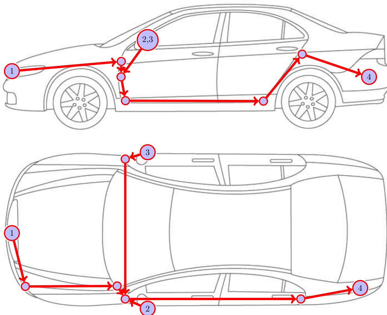
Figure 3: Vehicle overview
